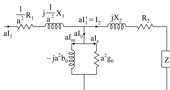
● 等效至二次側電路 ●
